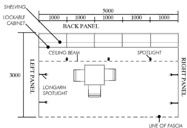
PLAN VIEW
